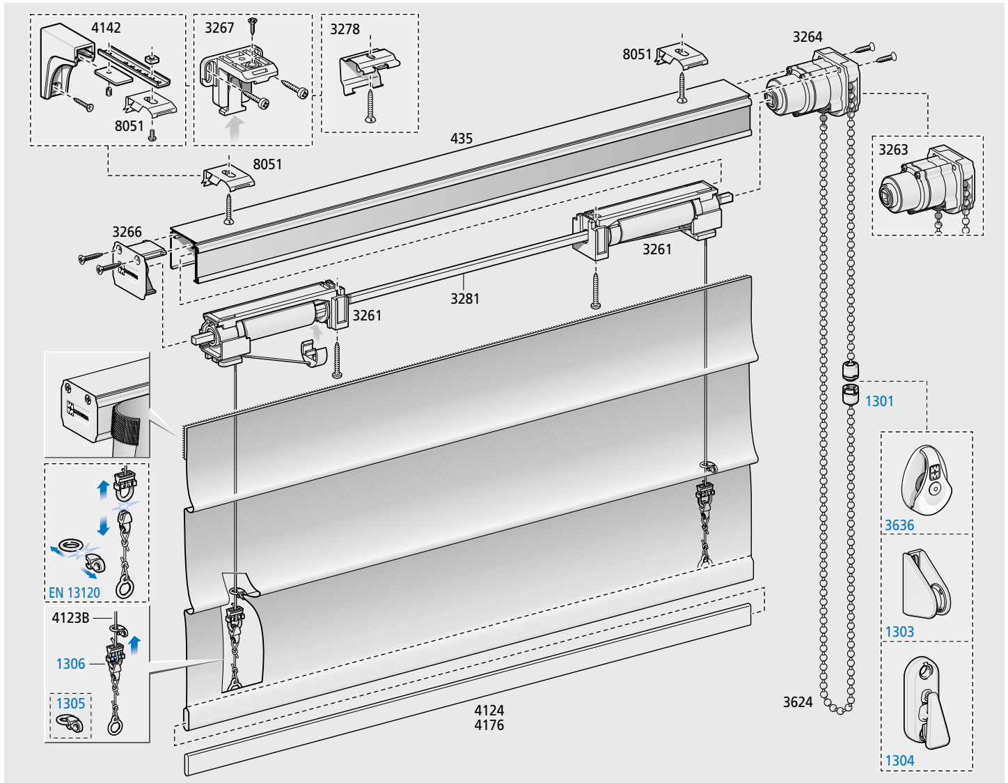
ROCCHETTO 3261 - REF. 3261 SPOOL - RECOGEDOR 3261 - BOBINE 3261 CASSETTE REF. 3261 - SPULEN 3261 - 3261 SPOELEN - БОБИНА 3261
